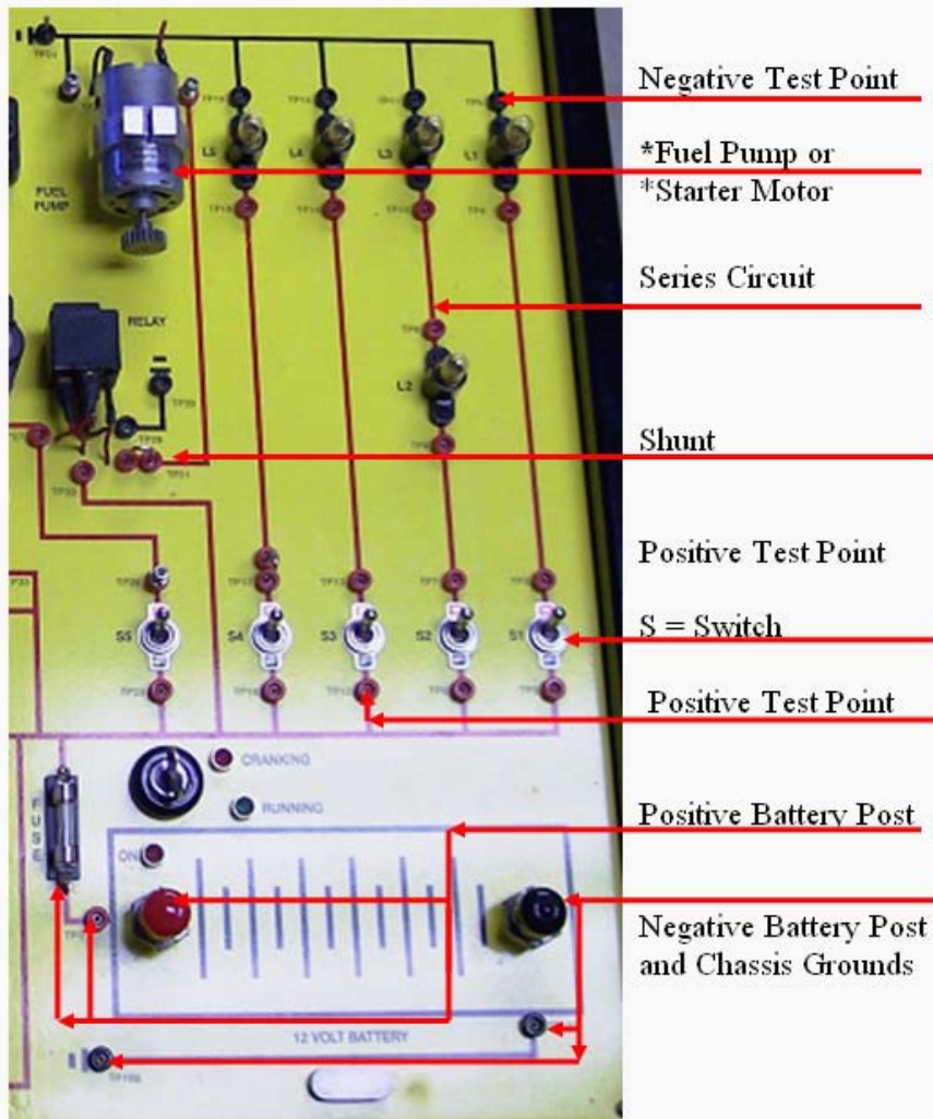
Description of ETrainer testing board
